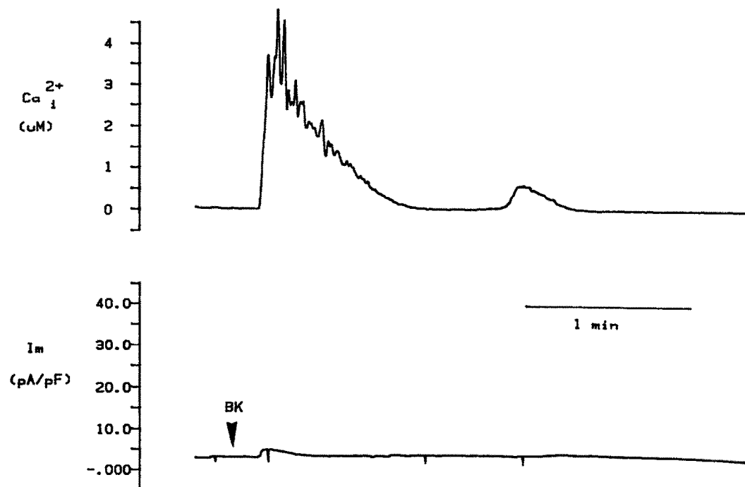
Fig.3. Response to BK from a cell loaded with Cs^+ (replacing K^+ ): in the upper trace, the Ca^{2+} concentration raises normally to micromolar levels, while the current ( V_h = +50 mV) shows only a very small increase (lower trace).
